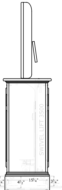
SIDE VIEW (THRU A)
