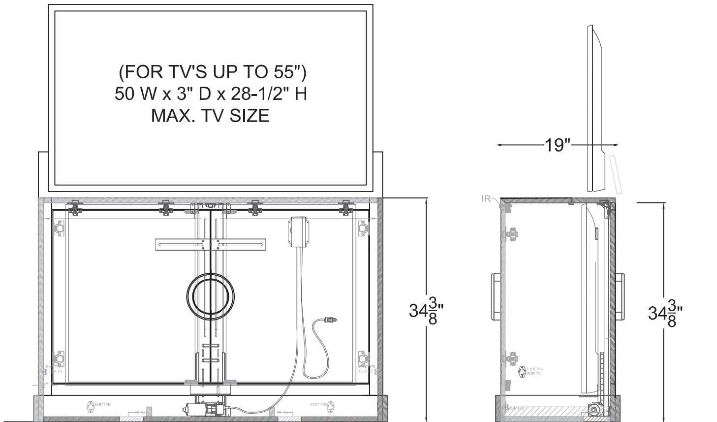
FRONT VIEW
